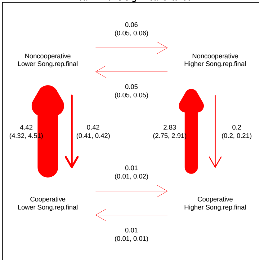
Thresholds \geq 1 - < 8.5 (23) Mean # Runs significant: 0/100
