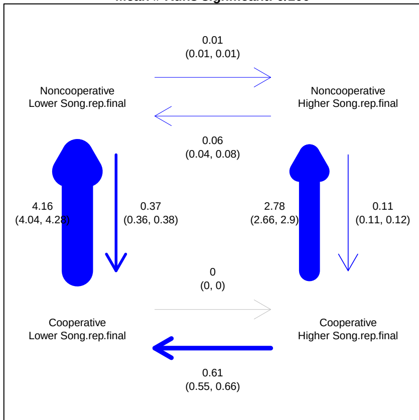
Thresholds \geq 34 - < 1450 (23) Mean # Runs significant: 0/100
