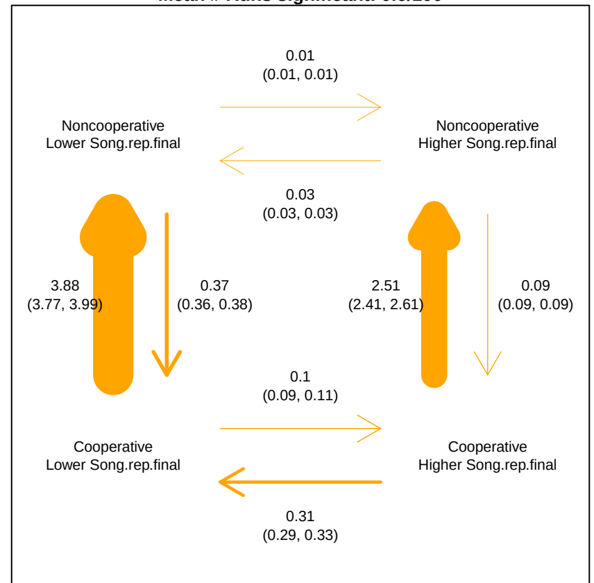
Thresholds \geq 8.5 - < 34 (24) Mean # Runs significant: 0.6/100
