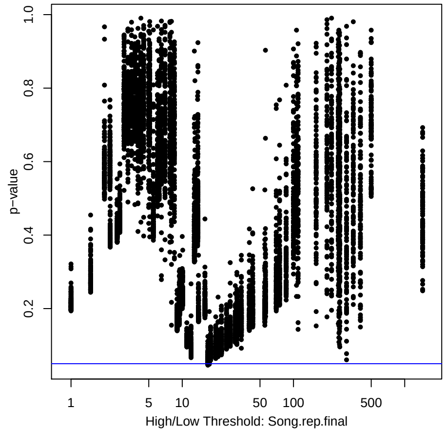
CoopBreed Song.rep.final Original threshold range: 1 - 1450 (70)
